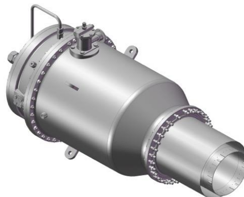
Figure 7: 3C Advanced diffusion type combustor for low calorific fuels
